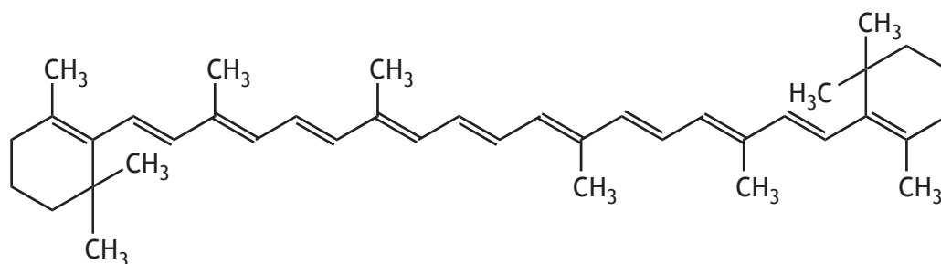
\beta -carotene
