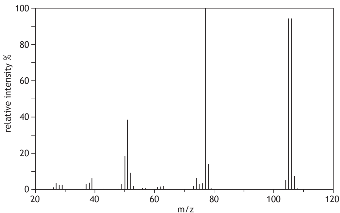
Mass Spectrum
