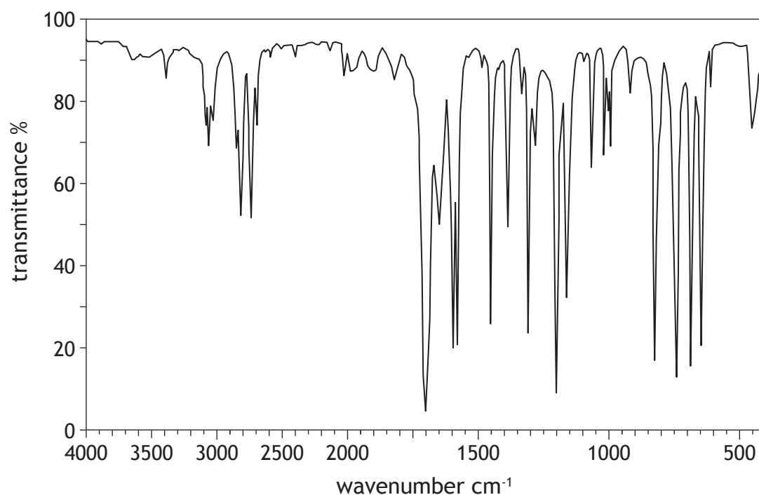
Infra-Red Spectrum
